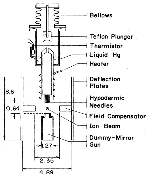
FIG. 3. Schematic diagram of the Hg gun (not to scale) and its positioning relative to the ion beam. Dimensions are in cm. The gun and its mirror image are kept at ground potential while the deflector plates have opposite polarities.
