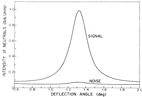
FIG. 5. Angular profile of neutral particles produced in electron loss of 134-keV H^- ions in passing through Hg vapor. The upper and lower curves were obtained with the Hg beam switched on and off. The signal profile is similar to the \theta=1.33^\circ distribution in Fig. 2.
