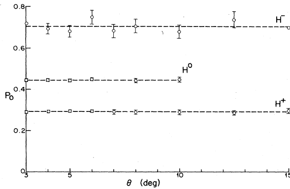
FIG. 6. Angular dependence of the fraction P_0 of neutral particles in Hg-scattered hydrogen projectiles for three incident beams of H^- , H^0 , and H^+ projectiles at an energy near 40 keV. Lines pass through the angle-averaged experimental points. Error bars are explained in the text.
