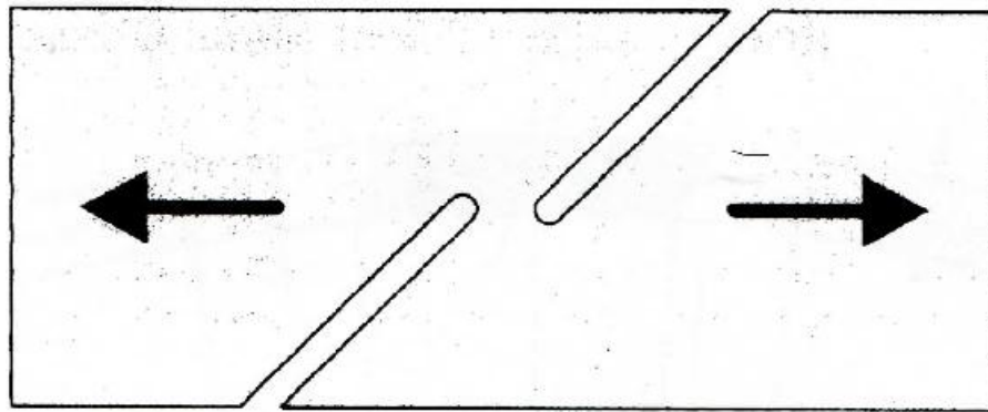
Figure 3.8 ASTM B831 shear test specimen for sheet materials [118]
