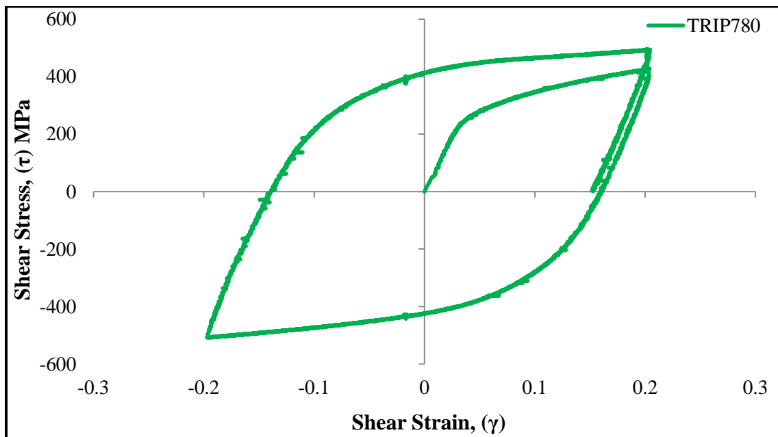
Figure 5.23 Experimental shear stresses - shear strains curves for TRIP780 steel
