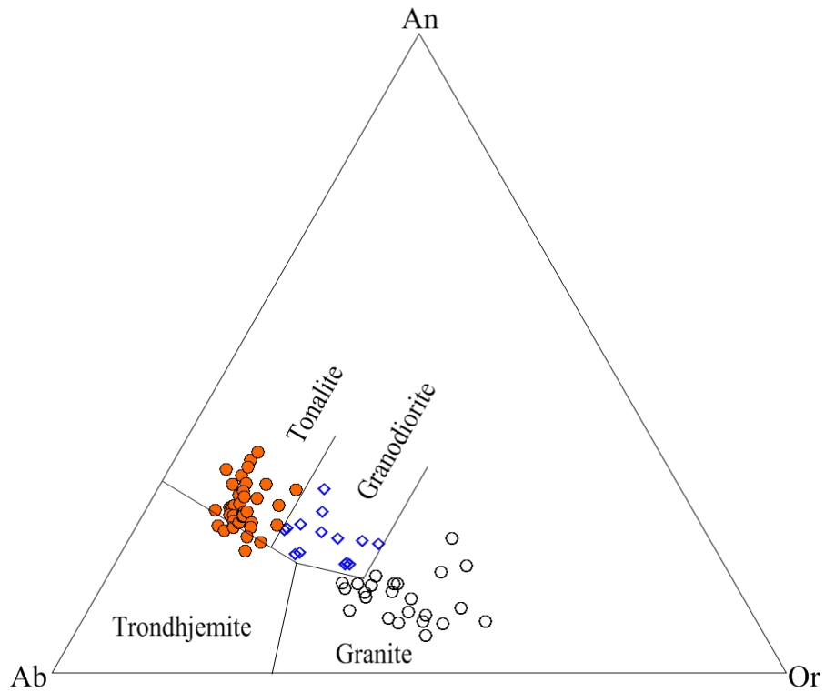
Fig 4.5. Classification of the granitoid gneisses using normative anorthite (an), albite (ab) and orthoclase (or), with fields defined by Barker (1979).
