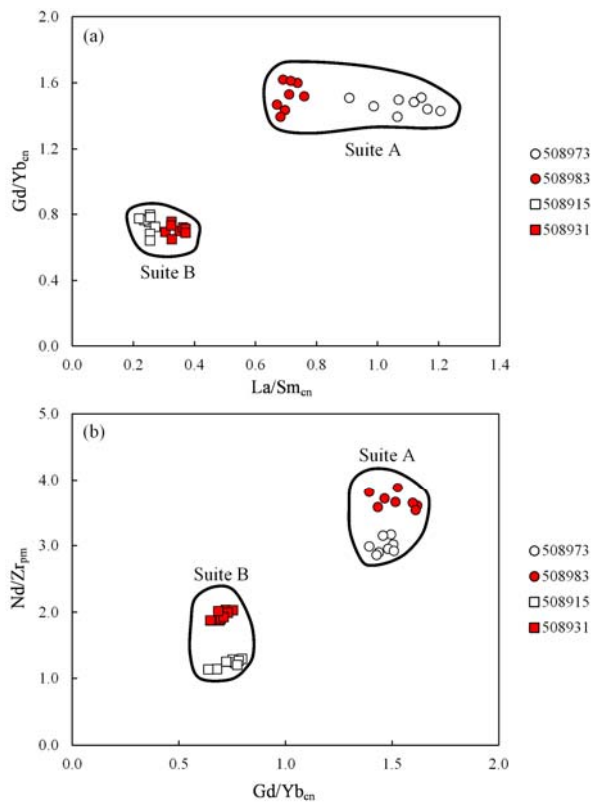
Fig. 2.9. (a) La/Sm_{cn} vs. Gd/Yb_{cn} and (b) Gd/Yb_{cn} vs. Nb/Zr_{pm} diagrams for hornblendes in the Ultramafic, Lower Gabbro, and Middle Gabbro Units. Chondrite normalization values are from Taylor and McLennan (1985) and N-MORB normalization values from Hofmann (1988).
