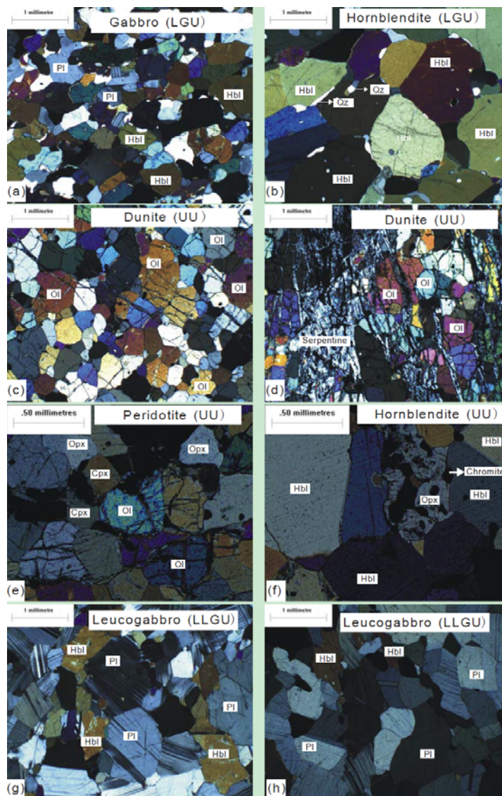
Supplementary Fig 2.2. Photomicrographs of the Lower Gabbro (LGU) Unit, Ultramafic Unit (UU) and Lower Leucogabbro Unit (LLGU) of the Fiskensæset Complex. (a) Gabbro with metamorphic plagioclase and hornblende. (b) Hornblendite with hornblende and quartz. (c) Dunite with olivine. (d) Dunite with olivine and serpentine. (e) Peridotite with olivine, orthopyroxene and clinopyroxene. (f) Hornblendite with hornblende, relict orthopyroxene and chromite. (g) Typical equilibrium texture with triple junctions with interfacial angles close to 120^\circ in leucogabbro with plagioclase and hornblende. (h) Leucogabbro with plagioclase and hornblende. (Pl: plagioclase, Hbl: hornblende, Qz: quartz, Ol: olivine, Cpx: clinopyroxene, Opx: orthopyroxene).
