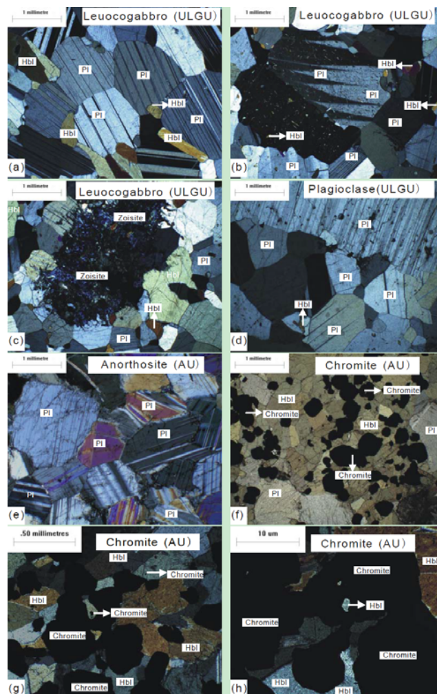
Supplementary Fig 2.4. Photomicrographs of the Upper Leucogabbro Unit (ULGU) and Anorthosite Unit rocks in the Fiskeneset Complex. (a) Typical equilibrium texture with triple junctions with interfacial angles close to 120^\circ in leucogabbro with plagioclase and minor hornblende. (b) Leucogabbro with twinned plagioclase and hornblende. Plagioclases contain tiny hornblende inclusions. (c) Leucogabbro with plagioclase (altered to zoisite) and hornblende. (d) Recrystallized plagioclases with stable equilibrium triple junctions and planar grain boundaries in Leucogabbro. (e) Anorthosite with plagioclase. (f) A chromite-rich layer in anorthosite. (g) Chromite inclusions in hornblende in anorthosite. (h) Hornblende inclusion in chromite in chromite. (Pl: plagioclase, Hbl: hornblende, Ol: olivine, Cpx: clinopyroxene, Opx: orthopyroxene).
