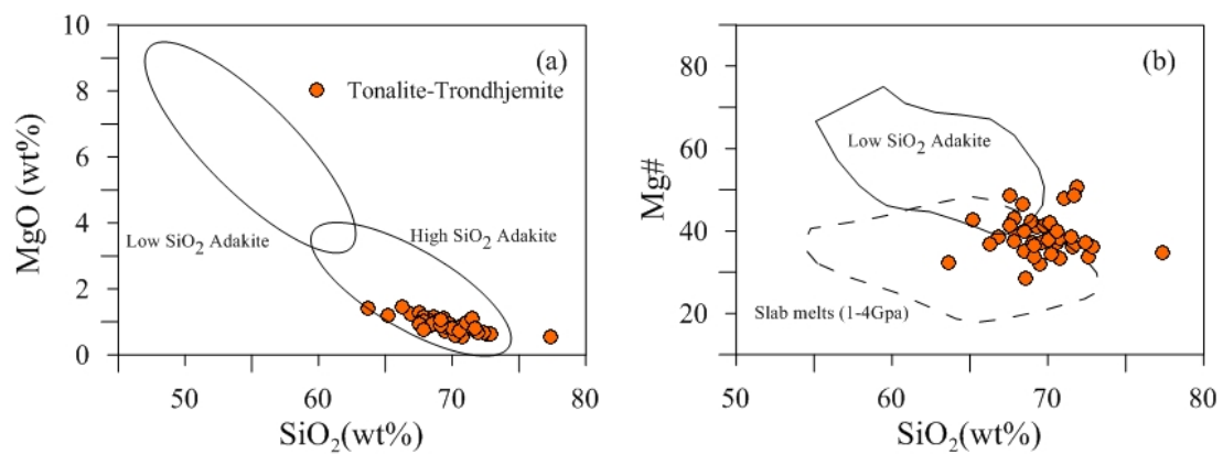
Fig 4.11. (a) SiO 2 vs. MgO for the tonalities and trondhjemites adapted from Martin (2005) and (b) SiO 2 vs. Mg# for the tonalities and trondhjemites adapted from Rapp et al. (1999) and Smithies (2000).
