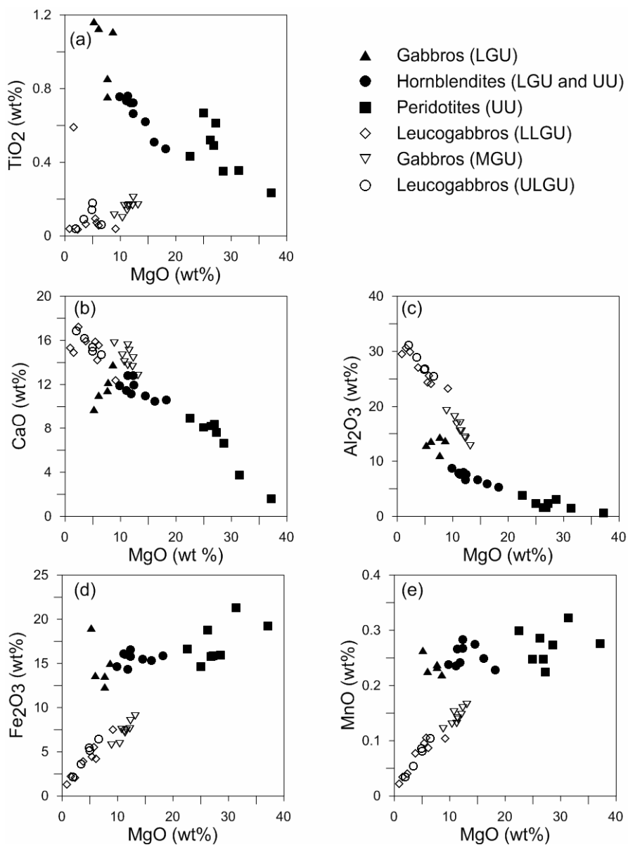
Fig. 2.4. TiO 2 , CaO, Fe 2 O 3 , MnO and Al 2 O 3 versus MgO variation diagrams for the Lower Gabbro Unit (LGU), Ultramafic Unit (UU), Lower Leucogabbro Unit (LLGU), Middle Gabbro Unit (MGU), and Upper Leucogabbro Gabbro (ULGU) Unit of the Fiskeneset Complex.
