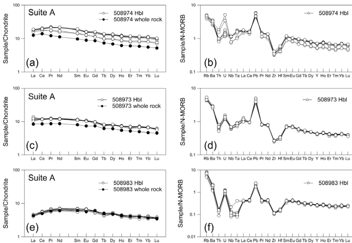
Fig 3.4. Chondrite-normalized REE and N-MORB-normalized trace element patterns for hornblende from gabbro (508974), and hornblendites (508973 and 508983) (Suite A).
