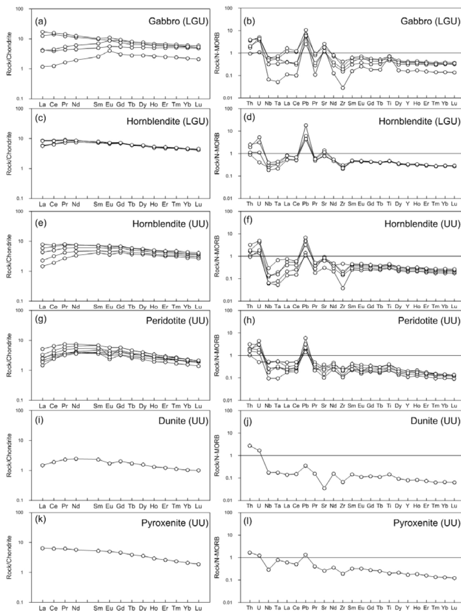
Fig. 2.5. Chondrite-normalized REE and N-MORB-normalized extended trace element diagrams for gabbro and hornblendite samples of the Lower Gabbro Unit (LGU) and for hornblendite, peridotite, dunite and pyroxenite samples of the Ultramafic Unit (UU). Chondrite normalization values are from Taylor and McLennan (1985) and N-MORB normalization values from Hofmann (1988).
