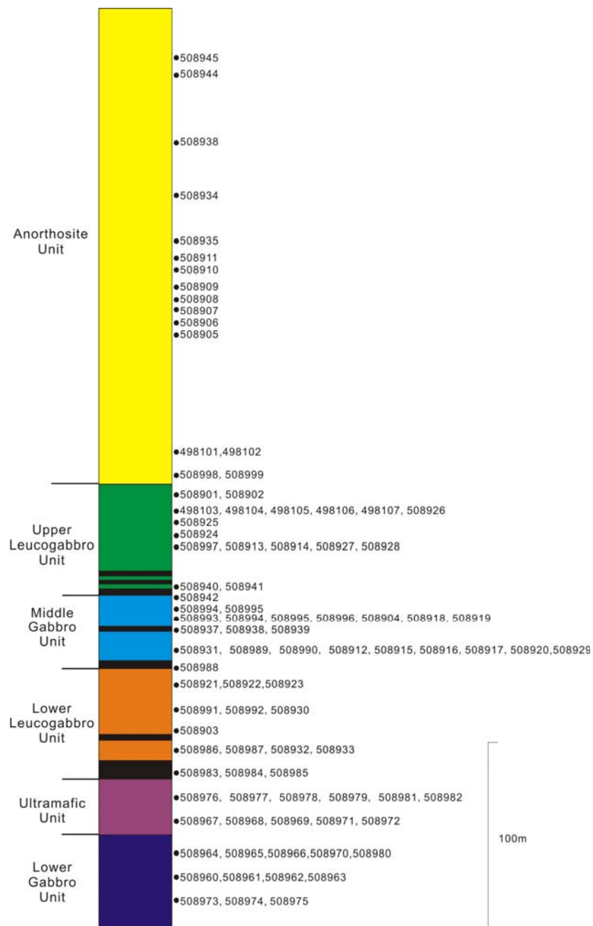
Supplementary Fig 2.1. Sample positions on the generalized stratigraphic section of the Fiskeneset Complex.
