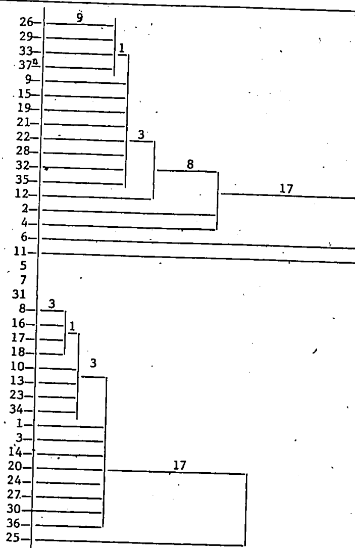
THE (K,R)-CLUSTERING DENDOGRAM GRAPH FOR THE H-CONFIGURATION
