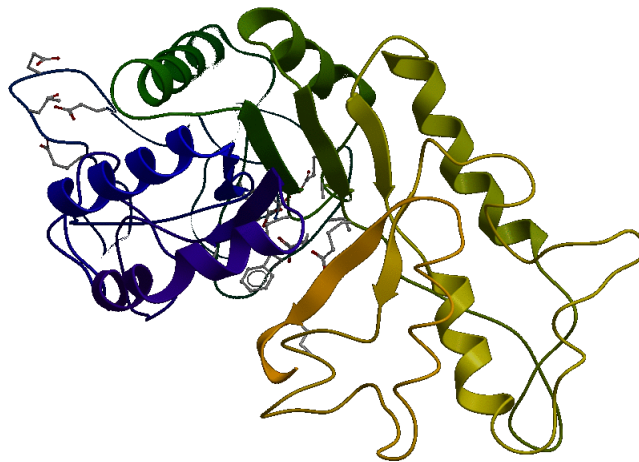
Figure 2.6: Representation of domains in complex PDB ID 1ava (chain A).
