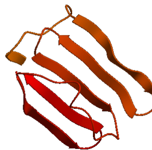
(b) Beta sheet
