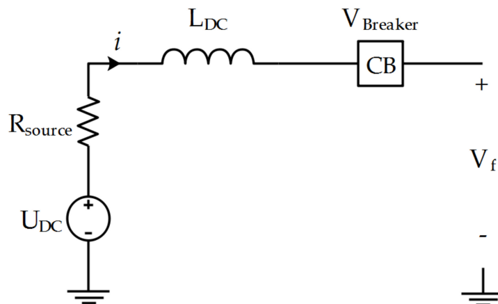
Figure 6. Configuration of the DC-link for fault analysis.
