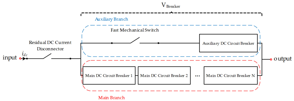
Figure 1. Overall structure of the proposed HDCCB.
