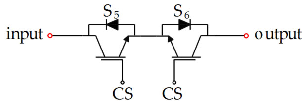
Figure 3. Configuration of the auxiliary DC CB.
