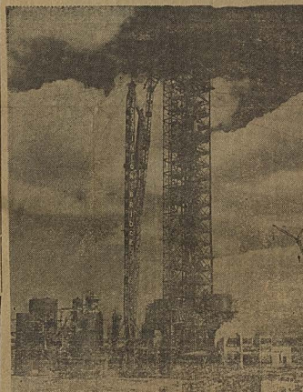
HIGH LATER: This new 100-ton derrick, part of its kind in Canada, towers 200 feet from ground to main top which means it can do a lifting job to a height much higher than Niagara Falls, anywhere in the country. Seen here in use for the first time, the derrick required five railcars to carry it from Lachine, Que., where it was built, to Sarnia, Ont. Here it was used to erect high oil cranking towers in building a new refinery.
