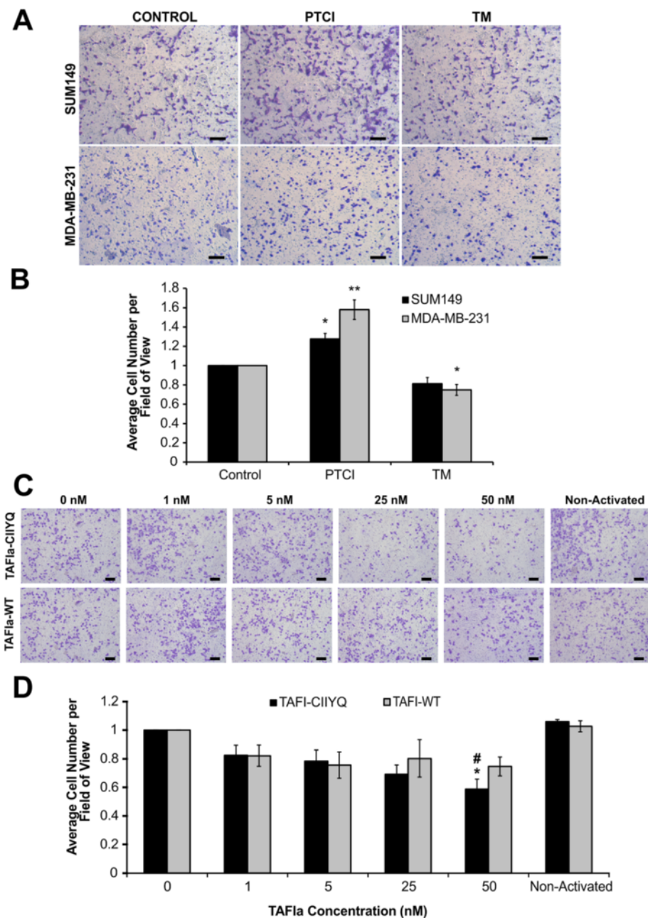
Fig. 4 The effects of PTCI, TM and TAFIa on breast cancer cell migration. a SUM149 and MDA-MB-231 cells were subjected to migration assays in the presence of 10 \mu\text{g}/\text{mL} PTCI or 10 nM TM or in the absence of these additions (Control). The number of migrated cells were imaged and counted in five fields of view. Images shown were taken at 4 \times magnification. Scale bars: 200 \mu\text{m} . b Quantification of migrated cells, relative to control (absence of treatment). The data represent the average cell number per field of view \pm SEM from at least 4 independent experiments. *: p < 0.05 and **: p < 0.01 relative to control. c Cells were treated with varying concentrations of either TAFIa-WT or TAFIa-CIIYQ (1–50 nM) for 24 h. Cells were also treated with 50 nM mock-activated TAFI-WT or TAFI-CIIYQ (Non-Activated). Migration was imaged as in (a). d Quantification of migrated cells, relative to control in the absence of TAFIa. The data represent the average cell number per field of view \pm SEM from at least three independent experiments. *: p < 0.05 relative to control; #: p < 0.05 relative to TAFIa-WT
