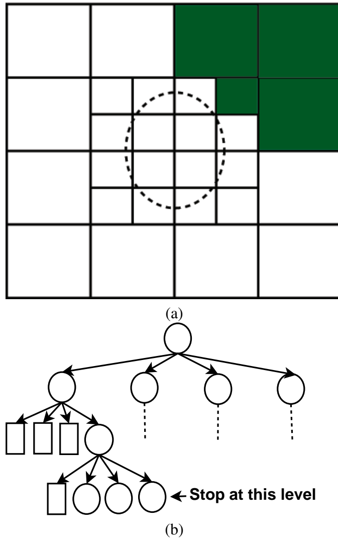
Figure 4.2: New signature representation method (a) A sample recursively divided image and (b) its corresponding quadtree
