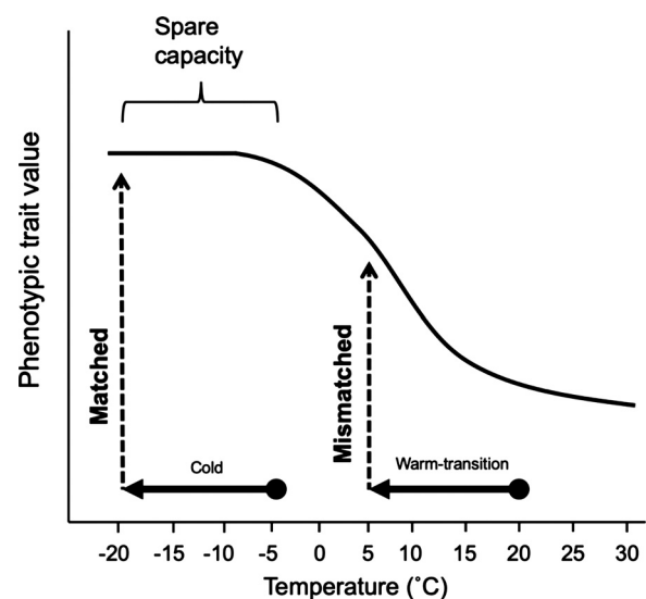
Fig. 1. Schematic representation of the reaction norm for phenotypic traits thought to covary with summit metabolic rate in response to ambient temperature ( ^{\circ}\text{C} ). Vertical dashed lines represent the matched (cold) and mismatched (warm-transition) phenotypes. The solid arrows represent the temperature drop for each group ( 15^{\circ}\text{C} each). Spare capacity is represented by the absence of change in a phenotypic trait for a given change in ambient temperature.
