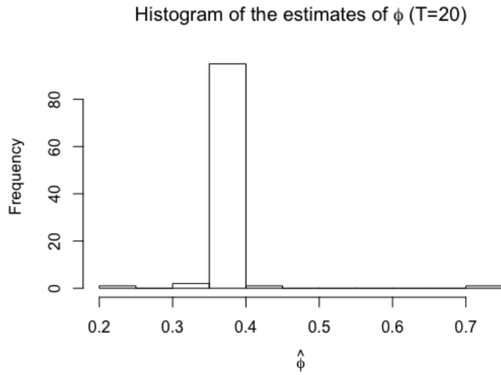
Figure 6.3: Histogram of the estimates of \phi for T=20
