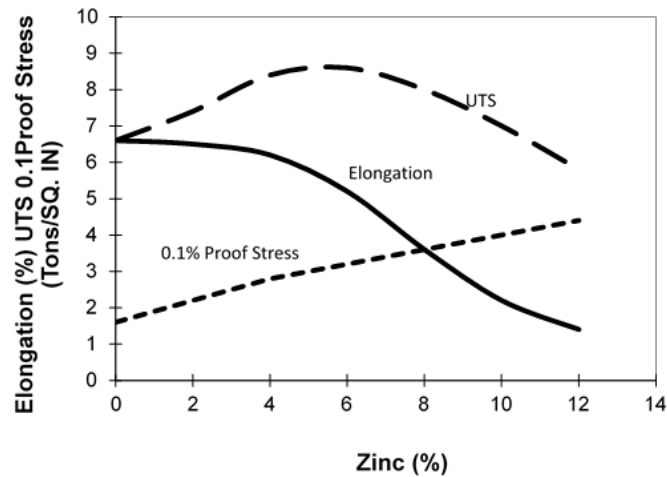
Figure 2.2 Tensile properties of sand cast (as-cast) Mg-Zn alloys [5].
