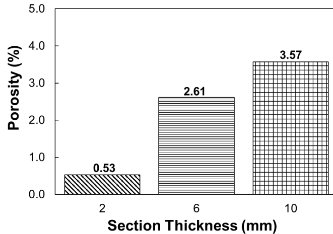
Figure 4.2 Porosity content vs. section thicknesses
