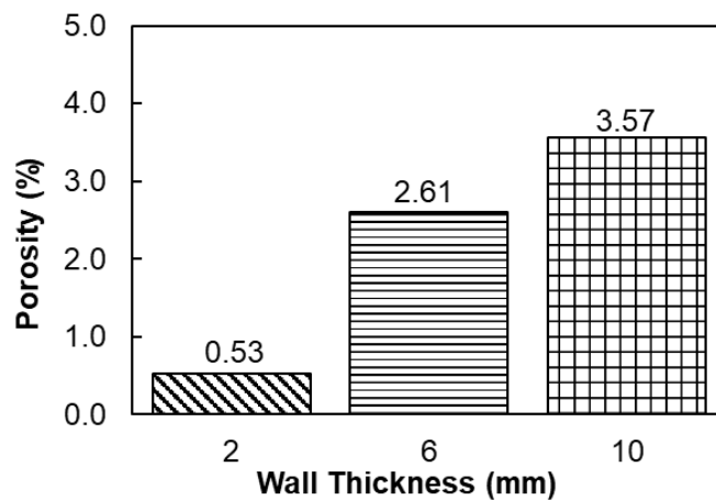
Figure 3.2 Porosity content vs. wall thicknesses
