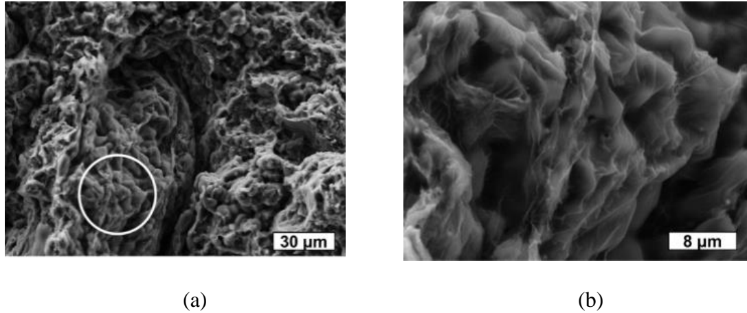
Figure 4.15 SEM fractographs of the 10 mm-thick die cast coupon, (a) low and (b) high magnification.
