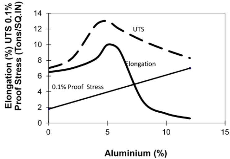
Figure 2.1 Tensile properties of sand cast (as-cast) Mg-Al alloys [5].
