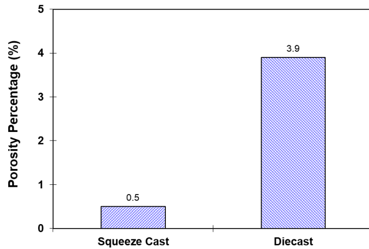
Figure 2.14 Porosity levels of squeeze cast and die cast AZ91D parts with 5 mm section thickness [33].
