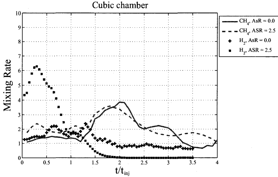
Fig. 4.28: Mixing rate vs. time at different swirl ratios in constant cubic volume chamber; CH_4 : U_{inj} = 150\text{ m/s} , t_{inj} = 10\text{ ms} , t_{sinj} = 0 ; H_2 : U_{inj} = 150\text{ m/s} , t_{inj} = 20\text{ ms} , t_{sinj} = 0 .
