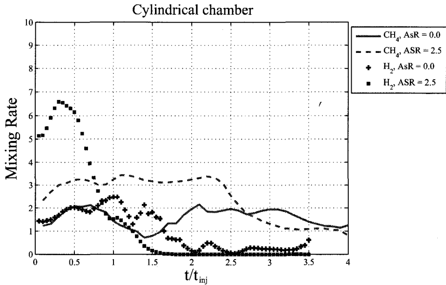
Fig. 4.29: Mixing rate vs. time at different swirl ratios in constant cylindrical volume chamber; CH_4 : U_{inj} = 150\text{ m/s} , t_{inj} = 10\text{ ms} , t_{sinj} = 0 ; H_2 : U_{inj} = 150\text{ m/s} , t_{inj} = 20\text{ ms} , t_{sinj} = 0 .
