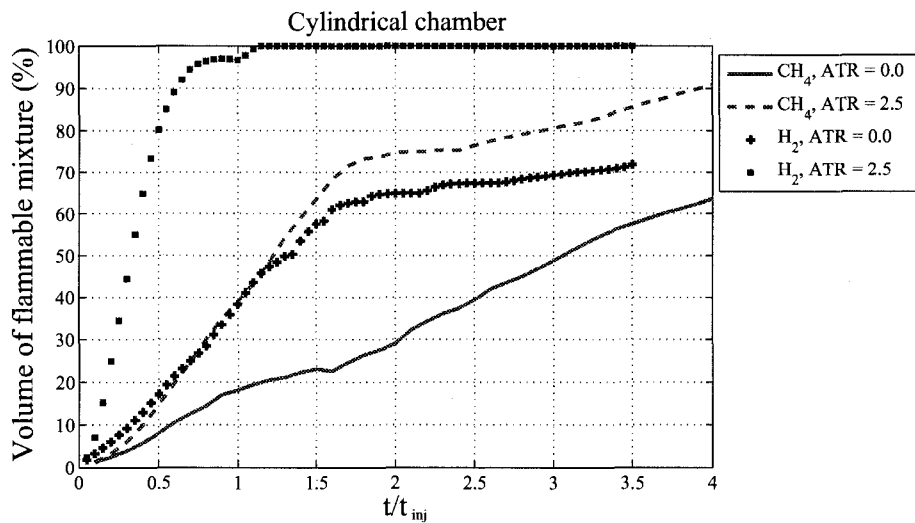
Fig. 4.15: Comparison of flammable mixture formation between H_2 and CH_4 at two different tumble ratios in cylindrical constant volume chamber; CH_4 : U_{inj} = 150 \text{ m/s} , t_{inj} = 10 \text{ ms} , t_{sinj} = 0 ; H_2 : U_{inj} = 150 \text{ m/s} , t_{inj} = 20 \text{ ms} , t_{sinj} = 0 .
