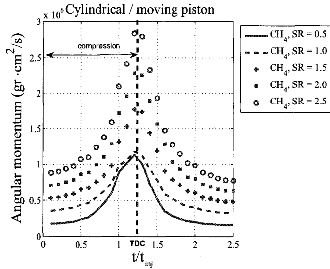
Fig. 4.40: Angular momentum change time at different swirl ratios in cylindrical chamber with moving piston; U_{inj} = 150\text{m/s} , t_{inj} = 10\text{ms} , t_{sinj} = 0 , calculated for the entire volume above the moving piston.
