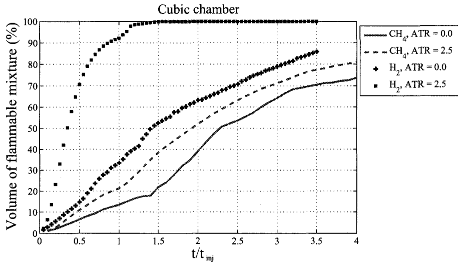
Fig. 4.14: Comparison of flammable mixture formation between H_2 and CH_4 at two different tumble ratios in cubic constant volume chamber; CH_4 : U_{inj} = 150 \text{ m/s} , t_{inj} = 10 \text{ ms} , t_{sinj} = 0 ; H_2 : U_{inj} = 150 \text{ m/s} , t_{inj} = 20 \text{ ms} , t_{sinj} = 0 .
