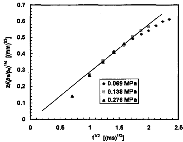
Fig. 2.4: Penetration depth vs. square root of time [2].
