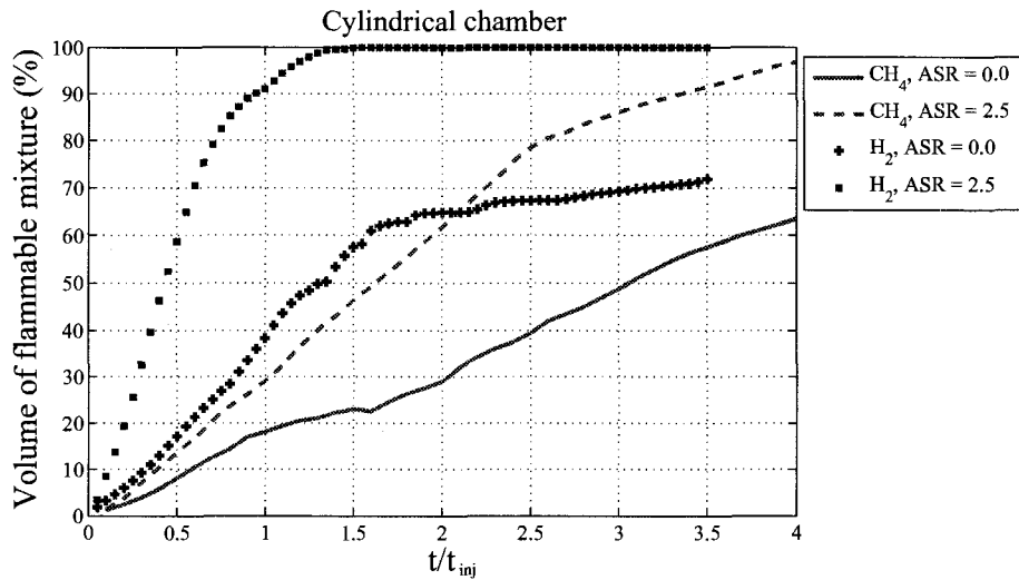
Fig. 4.13: Comparison of flammable mixture formation between H_2 and CH_4 at two different swirl ratios in cylindrical constant volume chamber; CH_4 : U_{inj} = 150\text{ m/s} , t_{inj} = 10\text{ ms} , t_{sinj} = 0 ; H_2 : U_{inj} = 150\text{ m/s} , t_{inj} = 20\text{ ms} , t_{sinj} = 0 .
