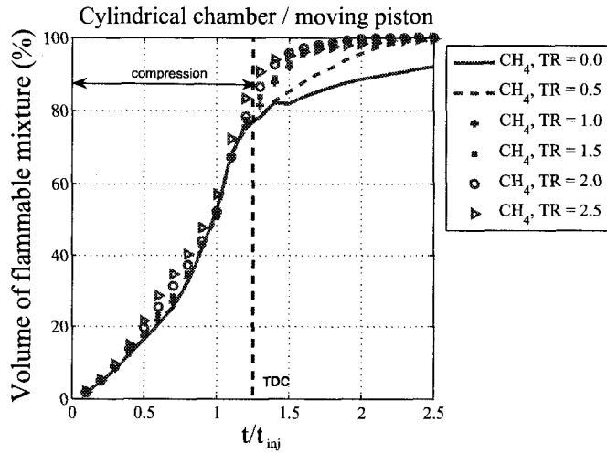
Fig. 4.17: Volume of flammable mixture vs. time at different tumble ratios in cylindrical chamber with moving piston; U_{inj} = 150\text{m/s} , t_{inj} = 10\text{ms} , t_{sinj} = 0 .
