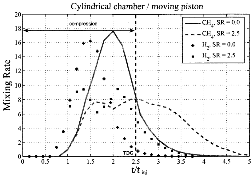
Fig. 4.34: Mixing rate vs. time at different swirl ratios in cylindrical chamber with moving piston; CH_4 : U_{inj} = 300m/s , t_{inj} = 5ms , t_{sinj} = 6.25ms ; H_2 : U_{inj} = 450m/s , t_{inj} = 6.6ms , t_{sinj} = 6.25ms .
