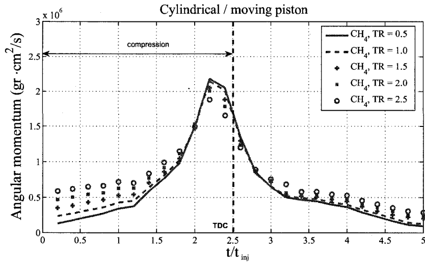
Fig. 4.43: Angular momentum change time at different tumble ratios in cylindrical chamber with moving piston. U_{inj} = 300m/s , t_{inj} = 5ms , t_{sinj} = 6.25ms , calculated for the entire volume above the moving piston.
