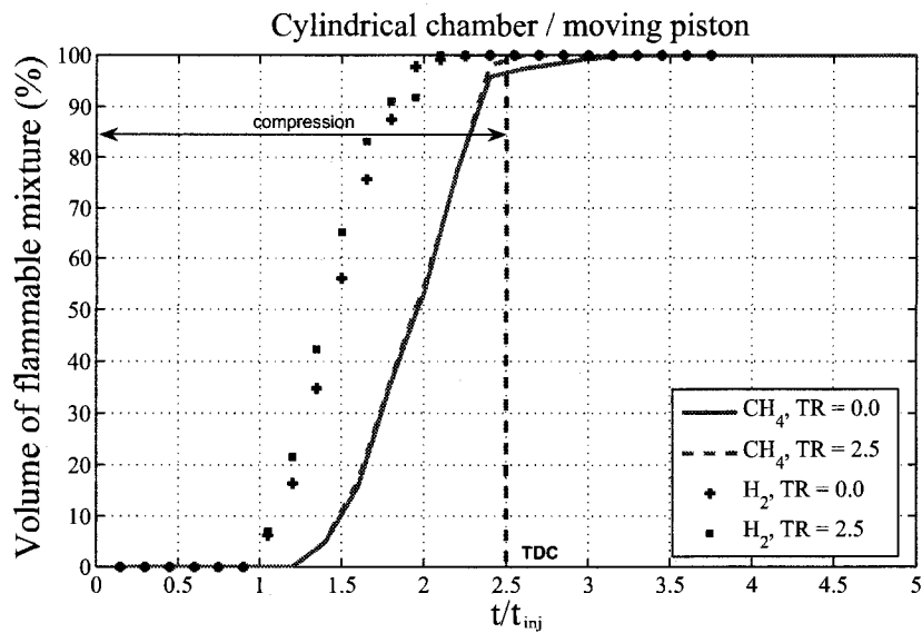
Fig. 4.27: Comparison of flammable mixture formation between H_2 and CH_4 at two different tumble ratios in cylindrical chamber with moving piston; CH_4: U_{inj} = 300m/s , t_{inj} = 5ms , t_{sinj} = 6.25ms ; H_2: U_{inj} = 450m/s , t_{inj} = 6.6ms , t_{sinj} = 6.25ms .
