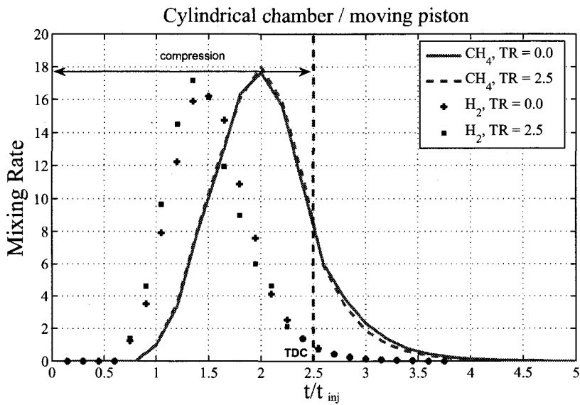
Fig. 4.35: Mixing rate vs. time at different swirl ratios in cylindrical chamber with moving piston; CH_4 : U_{inj} = 300m/s , t_{inj} = 5ms , t_{sinj} = 6.25ms ; H_2 : U_{inj} = 450m/s , t_{inj} = 6.6ms , t_{sinj} = 6.25ms .
