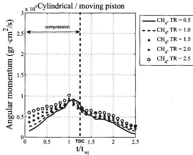
Fig. 4.41: Angular momentum change time at different tumble ratios in cylindrical chamber with moving piston; U_{inj} = 150\text{m/s} , t_{inj} = 10\text{ms} , t_{sinj} = 0 , calculated for the entire volume above the moving piston.
