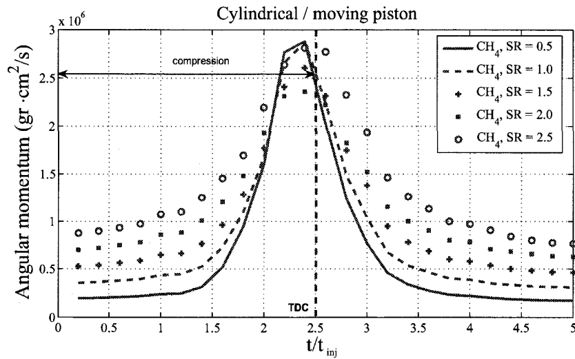
Fig. 4.42: Angular momentum change time at different swirl ratios in cylindrical chamber with moving piston. U_{inj} = 300m/s , t_{inj} = 5ms , t_{sinj} = 6.25ms , calculated for the entire volume above the moving piston.
