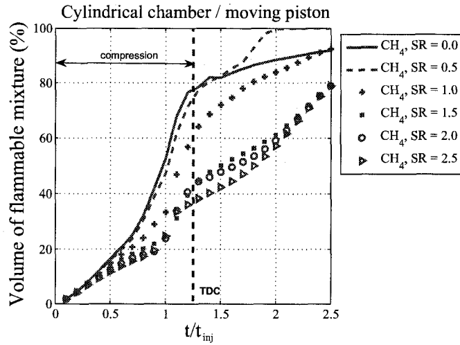
Fig. 4.16: Volume of flammable mixture vs. time at different swirl ratios in cylindrical chamber with moving piston; U_{inj} = 150\text{m/s} , t_{inj} = 10\text{ms} , t_{sinj} = 0 .
