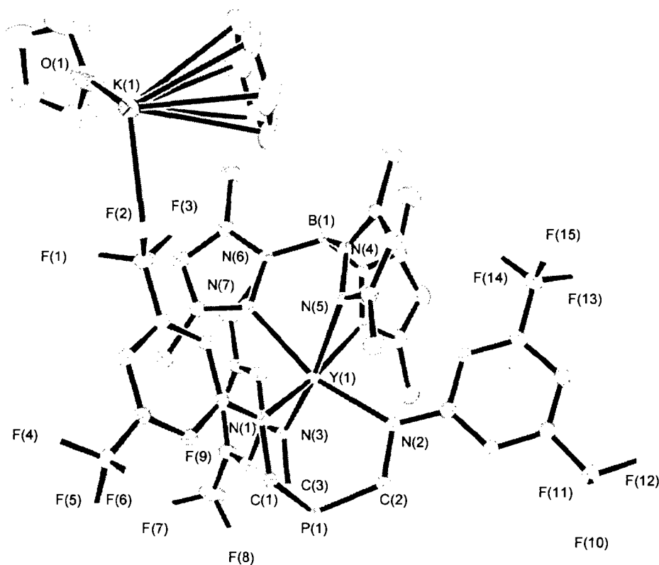
Figure 2.9. An ORTEP depiction of the solid-state molecular structure of K^+[P(CH_2N-3,5-(CF_3)_2C_6H_3)_3YTp^{Mc}]^- ( 12c ) showing potassium attached with cocrystallized benzene and THF. 30% thermal ellipsoids are shown. Hydrogen atoms are omitted for clarity and only the ipso carbons of the phenyl substituents on nitrogen are shown. Selected bond lengths or distances (Å): Y(1)---P(1), 3.3173(9); Y(1)---B(1), 3.543(5); Y(1)-N(3), 2.298(3); Y(1)-N(1), 2.292(3); Y(1)-N(2), 2.288(3); Y(1)-N(5) 2.432(3); Y(1)-N(7) 2.452(3); Y(1)-N(9), 2.453(3). Selected angles in degrees: N(7)-Y(1)-N(9), 78.81(9); N(5)-Y(1)-N(9), 74.49(9); N(5)-Y(1)-N(7), 77.61(9); C(3)-P(1)-C(1), 105.87(15); C(3)-P(1)-C(2), 106.96(15); C(1)-P(1)-C(2), 108.12(15).
