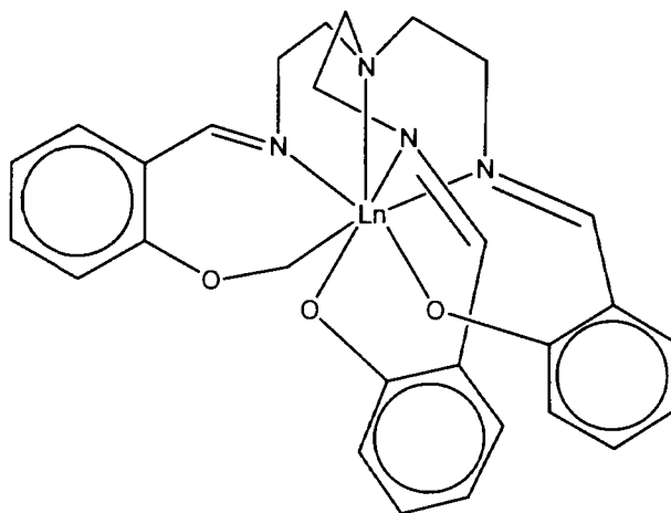
Figure 4.6. Schematic diagram of Ln(trensal) where Ln = Ce-Yb.
