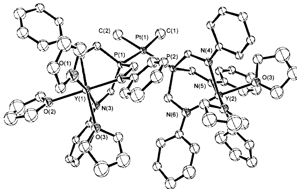
Figure 2.6. An ORTEP depiction of solid state molecular structure of [P(\text{CH}_2\text{N}-3,5\text{-(CF}_3)_2\text{C}_6\text{H}_3)_3\text{Y}(\text{THF})_3]_2\text{PtMe}_2 ( 9 ). Hydrogen atoms and \text{CF}_3 groups are omitted for clarity. Selected bond lengths or distances ( \text{\AA} ): \text{Y}(1)\cdots\text{P}(1) , 3.394(10) ; \text{P}(1)\text{--Pt}(1) , 2.287(7) ; \text{Y}(1)\cdots\text{Pt}(1) , 5.677(7) ; Selected angles in deg: \text{P}(1)\text{--Pt}(1)\text{--P}(1) , 97.7(3) ; \text{C}(1)\text{--Pt}(1)\text{--C}(2) , 81.8(17) .
