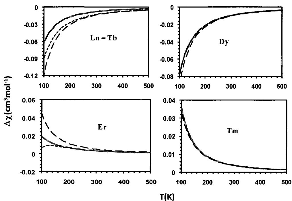
Figure 4.15. Comparison plot of temperature dependent magnetic anisotropies ( \Delta\chi ) calculated from Bleaney's (big dashed line), McGarvey's methods (small dashed line) and CONDON (grey line) vs temperature (T) for the C_{3h} symmetric lanthanide system.
