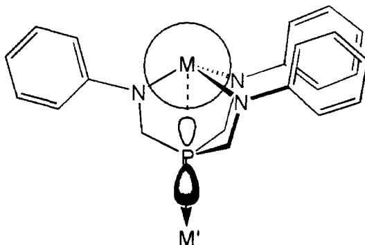
Figure 3.1. Through-space interactions in tripodal complexes of P(CH_2NPh)_3 with metal complexes M and M' with the minor and major lobes of lone pair orbital on phosphorus.
