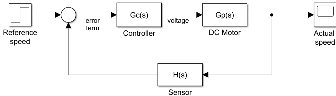
Figure 4.13: Closed-loop block diagram for DC motor control
