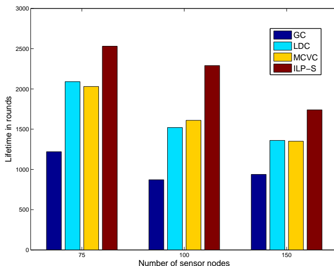
Figure 4.1: Comparison of network lifetimes with different clustering methods for a 12 relay node network under the single-hop routing scheme.
