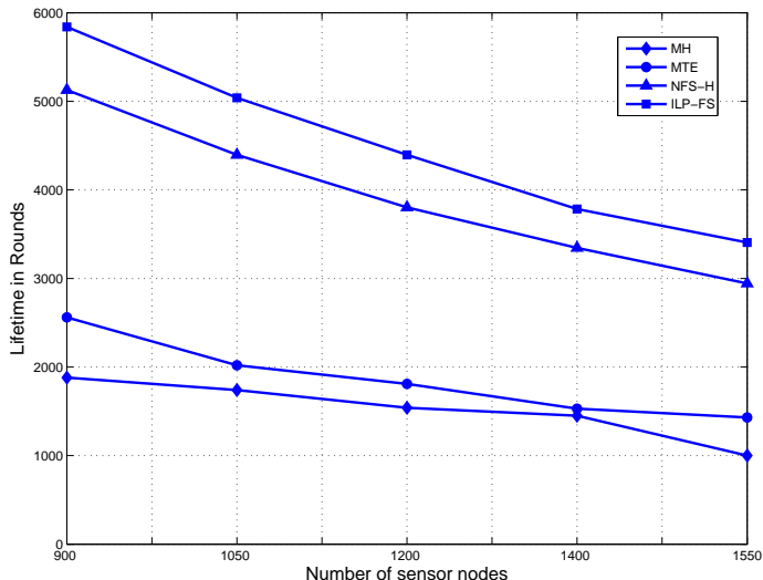
Figure 5.6: Comparison of achieved lifetimes for network with 36 relay nodes.
